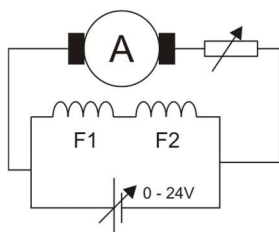
Circuit in use
