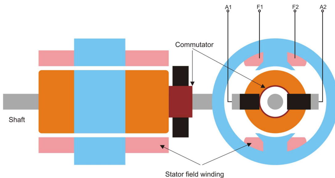
Construction
