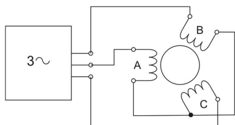
Circuit
