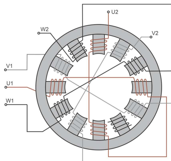
Stator winding circuit
