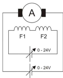
Conventional symbol
