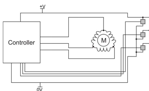
Conventional symbol
