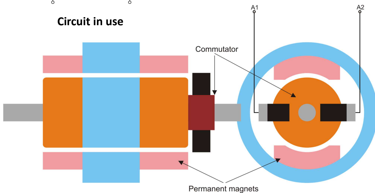
Construction
