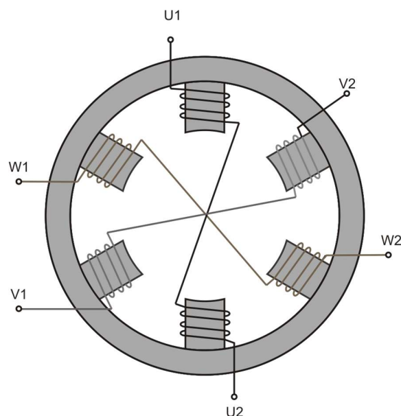
Stator winding circuit
